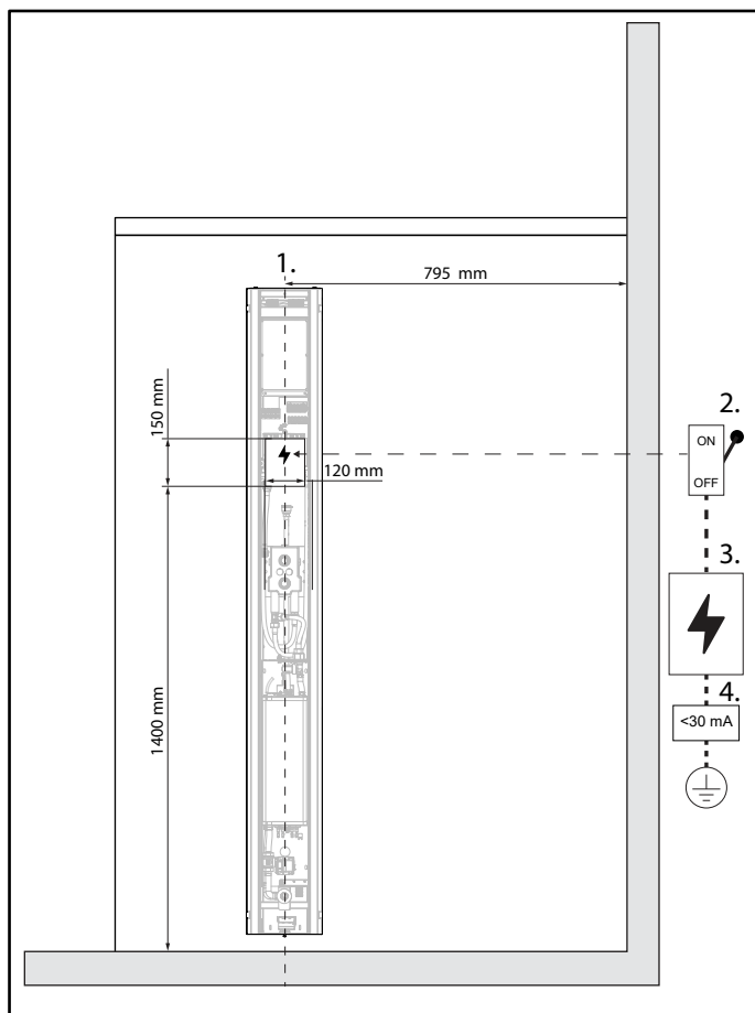
Fig. 6 Main power switch
