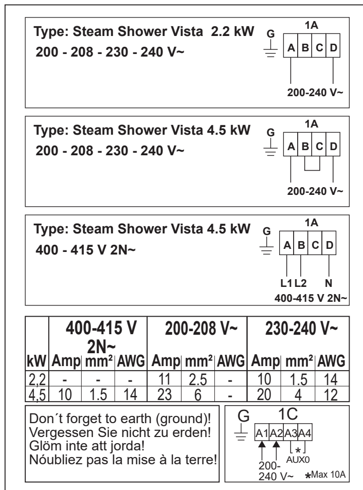
Fig. 7 Connections diagram
