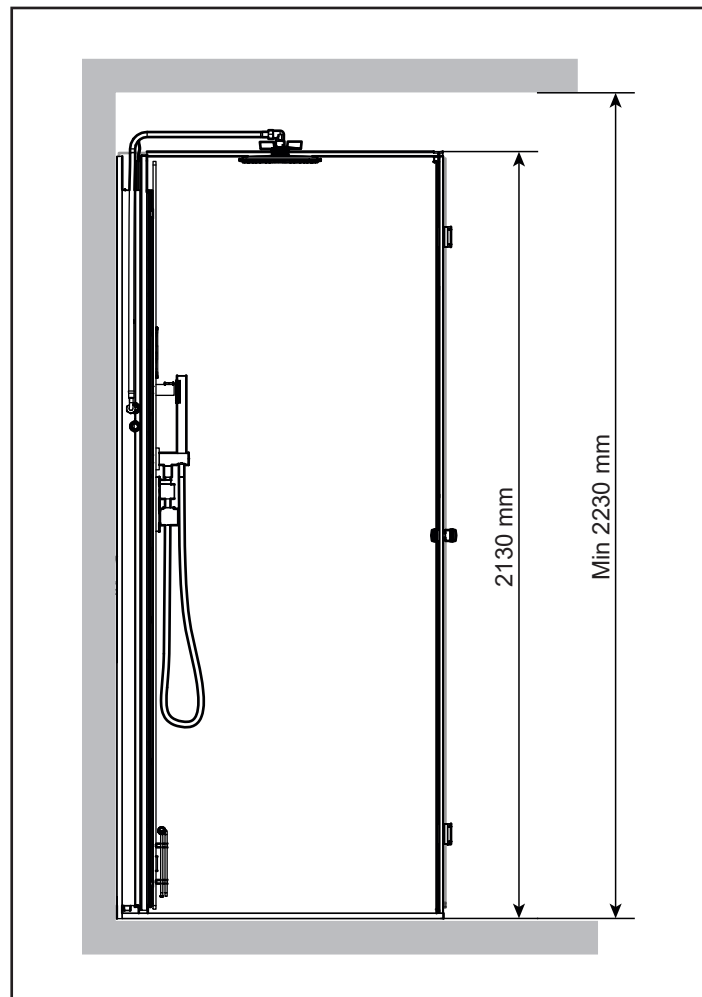
Fig. 2 Height dimensions Vista
